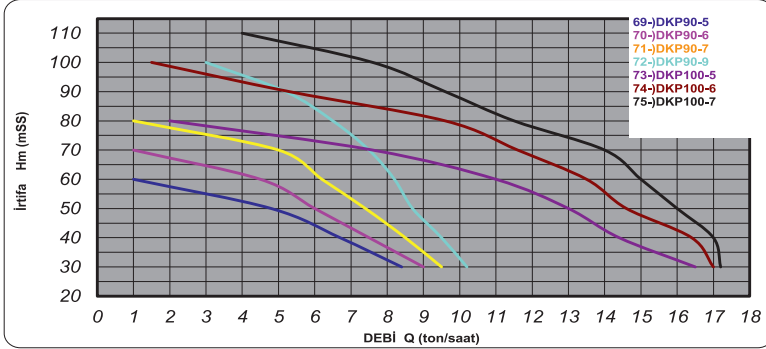
PERFORMANS EĞRİLERİ - PERFORMANCE CURVES
